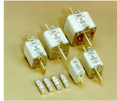
Fuses
